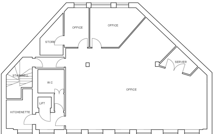
SECOND FLOOR Gross Internal Area 155.2 Sqm
