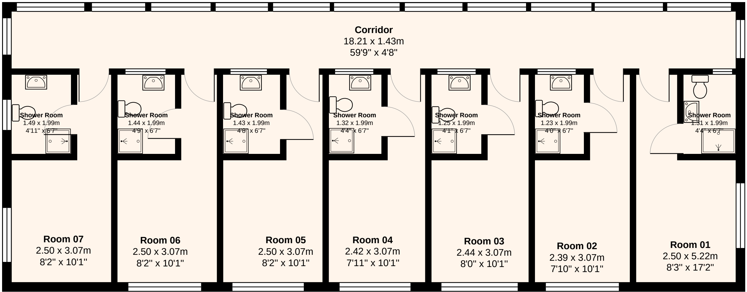
The Old Lamb Hotel First Floor
