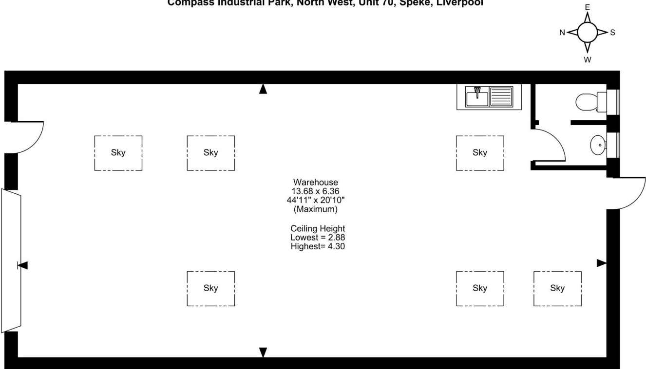
Ground Floor
