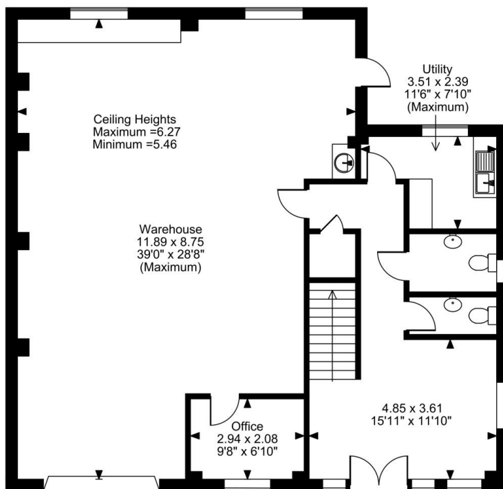
Ground Floor Roller Shutter Height = 4.32 Width = 3.01
