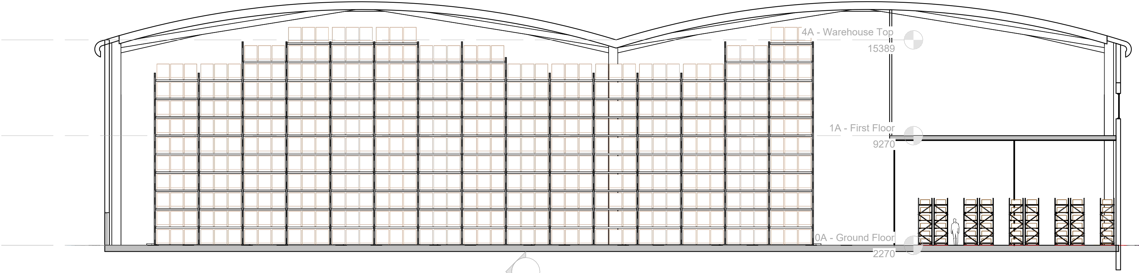
Section View
