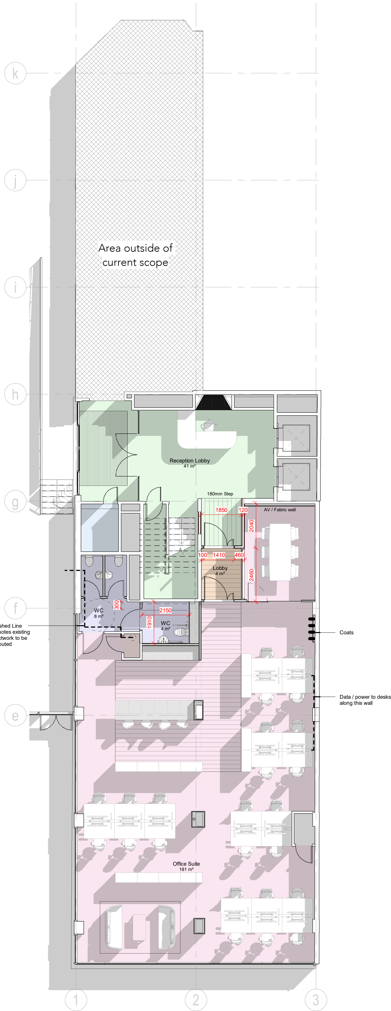
Level 0 Proposed Plan 1 : 100
